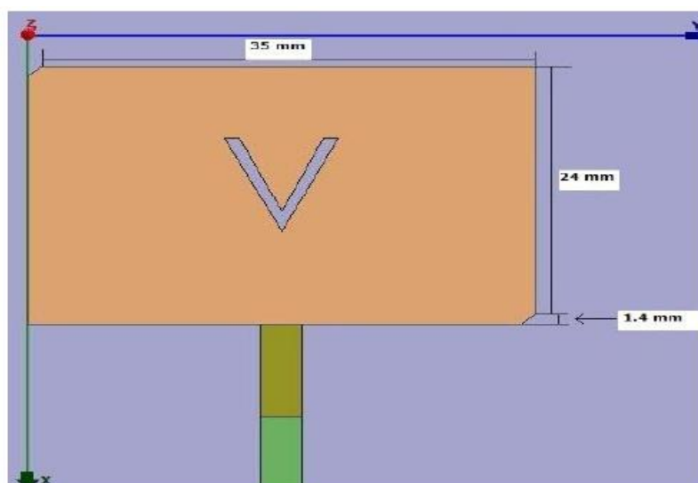
Figure 1: Corner truncated V-slotted patch antenna.
