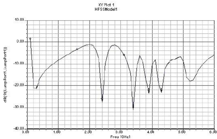
Figure 3: Simulated return loss of v-slotted rectangular patch antenna with truncation.
