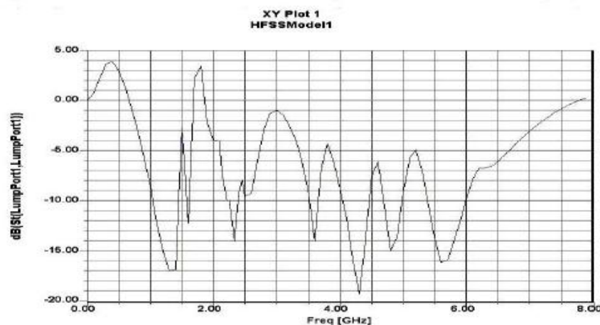
Figure 2: Simulated return loss of v-slotted rectangular patch antenna without truncation.
