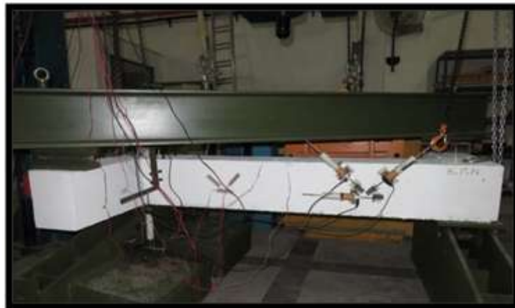
Fig.2.Experimental set-up of the beams
