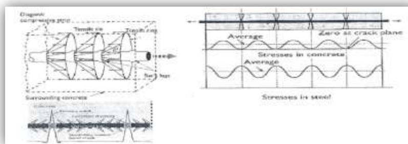
Fig.1.Effect of conical bond action of the stress in the reinforcement (2)
