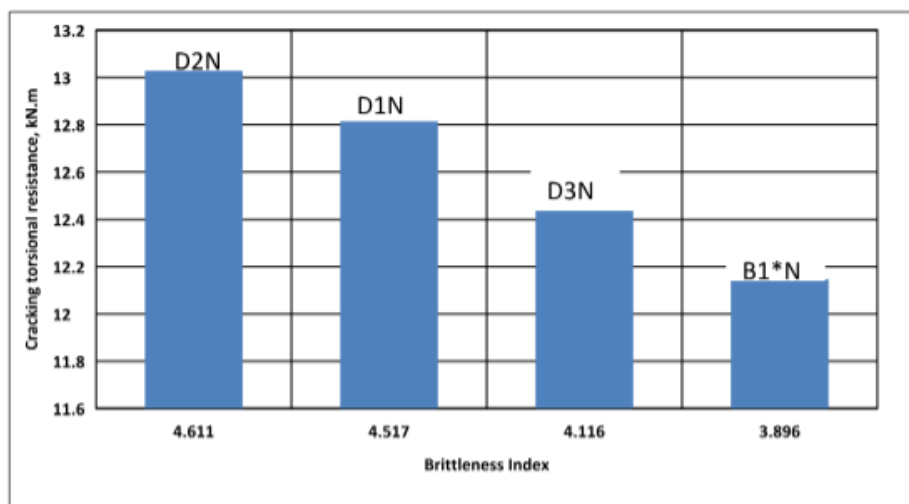
Fig.5. Cracking torsional resistance versus brittleness index
