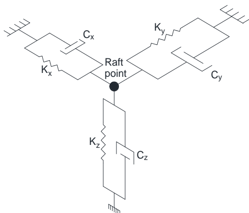
Fig.4: 3D view of the soil element
