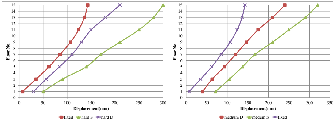
i) Lateral displacement for hard soil
