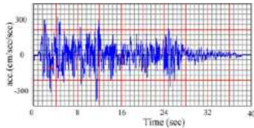
Fig.1: Earthquake wave El-Centro
