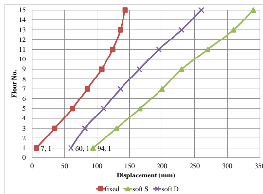
iii) Lateral displacement for soft soil
