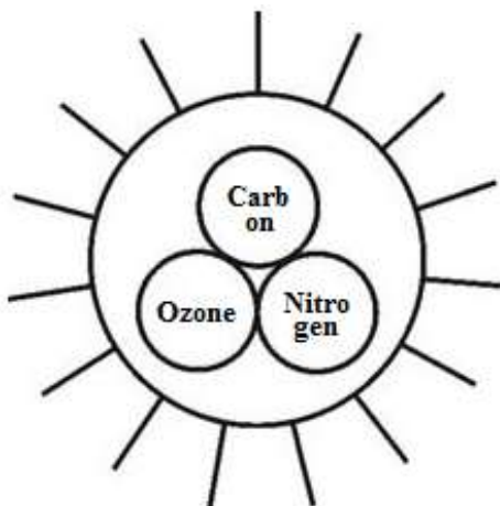
(Model Atom)
