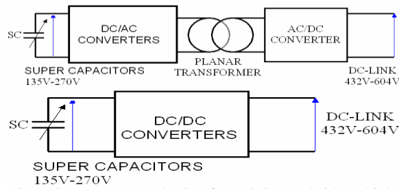
Fig1: Converter topologies for ECCE Hybrid Vehicle
