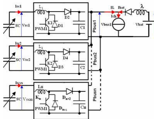
Fig 2(a): Multi boost Converter topology
