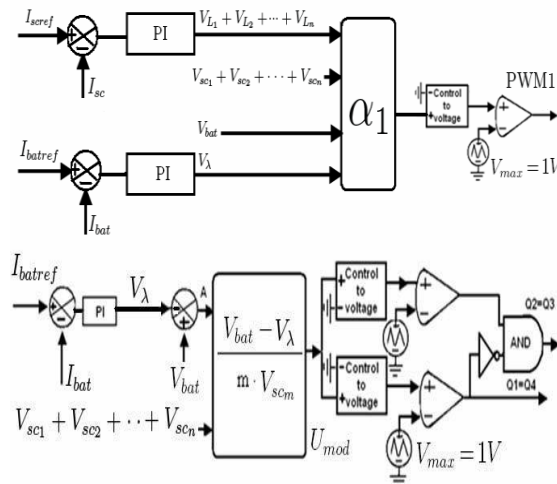
Fig 3. Multi boost and Multi full bridge converters control strategy
