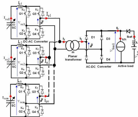
Fig 2(b): Multi full bridge converter topology
