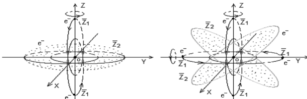
Figure 18.2 atomic surface 3 electron Figure 18.6 atomic surface 5 "s+p-type electron cloud" to form "s+p-type electron cloud" to form
