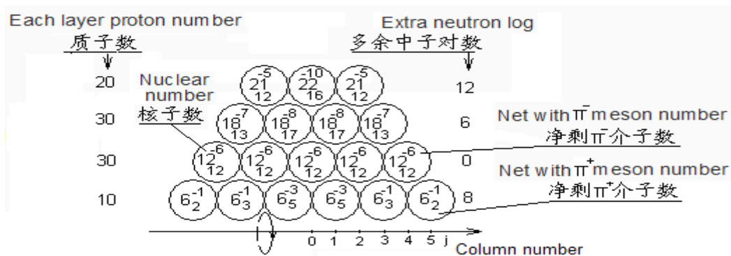
Figure 11.4 232 90 Th nucleus kernel sub、 net surplus \pi^{\pm} meson assigned to schematic diagram
