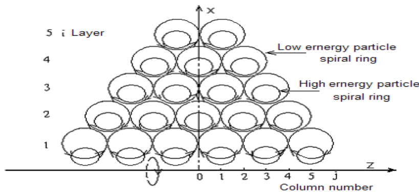
Figure 7.2 B nuclei internal low energy particles spiral ring combination schematic cross sectional view
