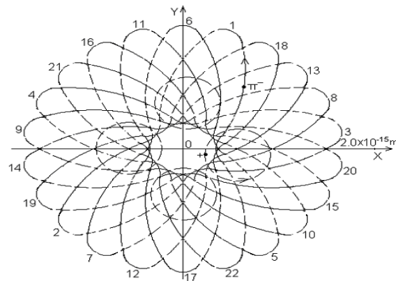
Fluctuations of the Figure 6.5 neutrons internal two electrically charged elementary particles spin motion track In XOY plane projection diagram
