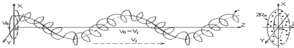
Figure 1.2 elementary particles along fluctuations, the spin precession of the orbital motion characteristics of the formation of wave-particle duality diagram
