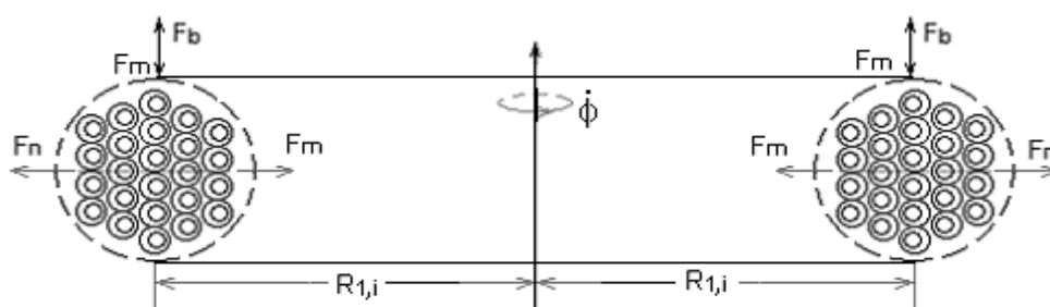
Figure 24.5 massive black hole internal neutron matter ring structure and gravitational F_m , the centrifugal force of the F_n nuclear force F_b balance diagram
