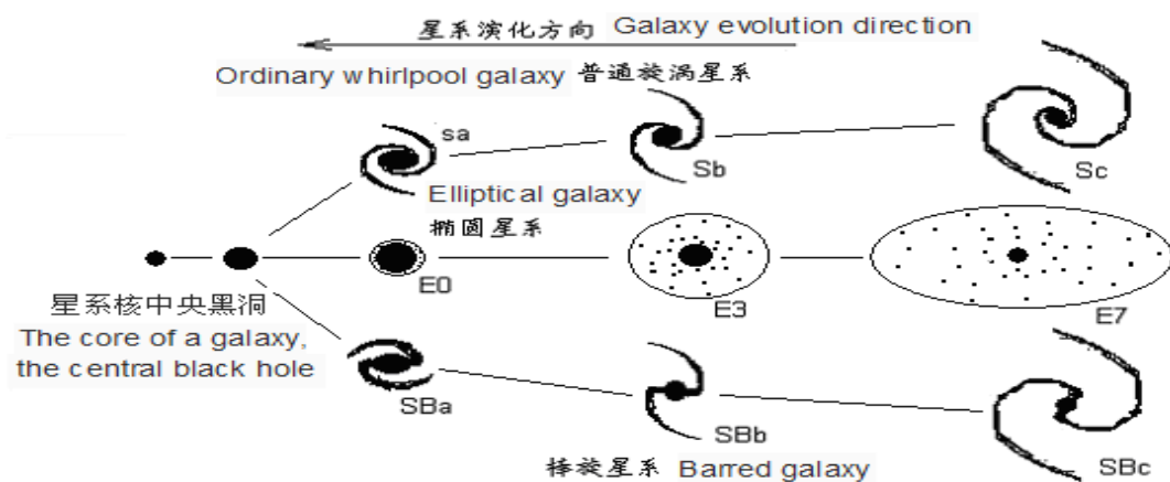
Figure 26.1 galaxy Hubble classification, evolution direction diagram
