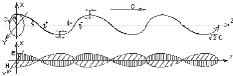
Figure 2.4 photons along fluctuations precession of the orbital motion of the medium wave-particle duality and electromagnetic waves forming principle schematic diagram
