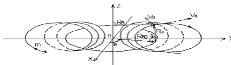
Figure 1.1 still elementary particle fluctuations, spin vertical double oval track movement diagram
