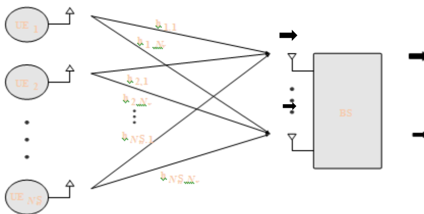
Figure 2: Uplink multiuser MIMO receiver model structure.
