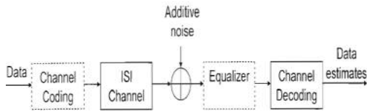
Figure 1: Baseband receiver model
