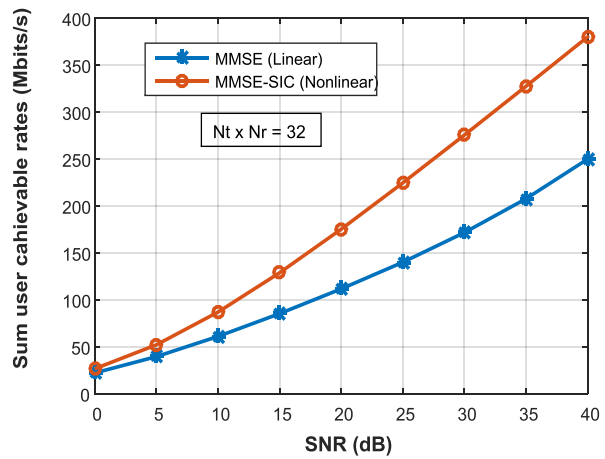
Figure 4c: User achievable rates versus SNR for MMSE and MMSE-SIC with N_t \times N_r = 3
