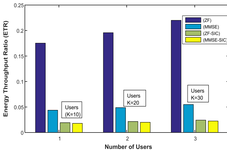
Figure 7: Energy throughput Ratio performance of ZF, MMSE, ZF-SIC and MMSE-SIC for N_t \times N_r fixed at 10, 20 and 30
