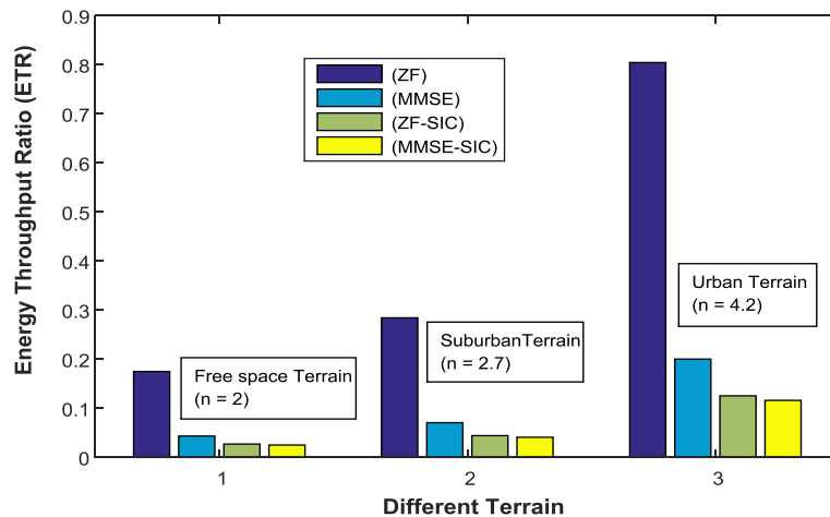
Figure 9: Energy throughput Ratio performance of ZF, MMSE, ZF-SIC and MMSE-SIC for n fixed at 2, 2.7 and 4.2
