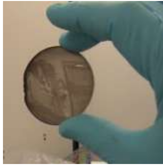
Figure 2. Free standing polycrystalline diamond, ~50 mm diameter and ~230 \mu\text{m} thick.
